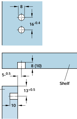
Drilling diagram
