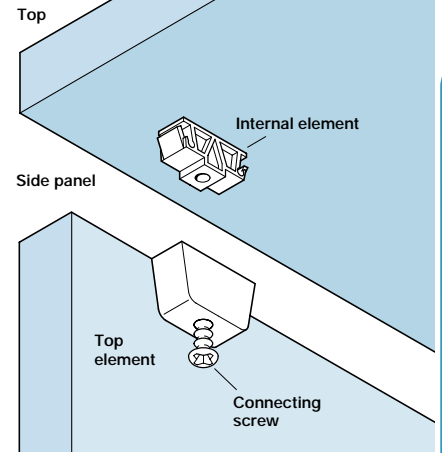
Mounting diagram
